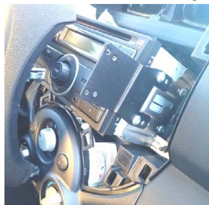
InDash Bottom Piece in place
